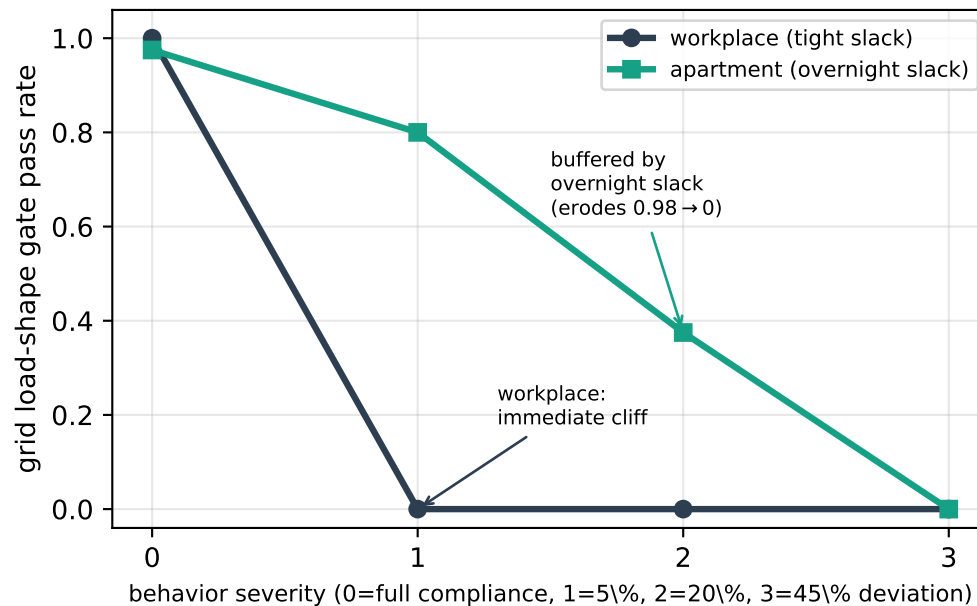
(A) The apartment grid benefit is compliance-contingent: coordination flattens the grid only while residents comply
