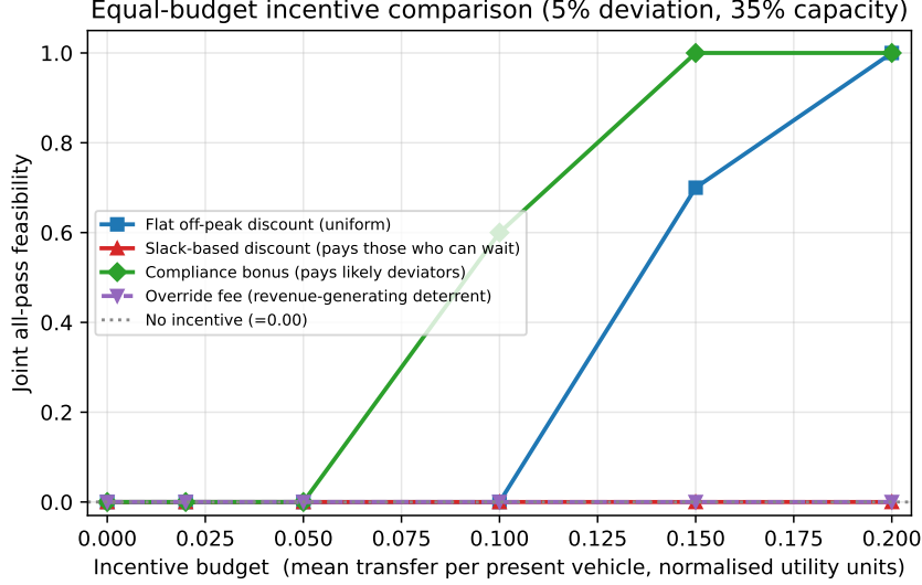
Figure 13: Equal-budget incentive comparison at the collapse point (5% deviation, 35% charger capacity, both grid settings, five seeds). All allocation rules spend the same average transfer per present vehicle (horizontal axis, normalised utility units). A compliance bonus targeted at the drivers most likely to override restores joint all-pass feasibility at a smaller budget than a uniform off-peak discount, whereas a slack-based discount that pays drivers who can already wait never restores it. A revenue-generating override fee (dashed) deters some deviation without spending budget but, at a strength matched to the flat discount, does not clear the compliance cliff and shifts cost onto drivers. Curves reflect the modelled compliance response, not measured field elasticities.
