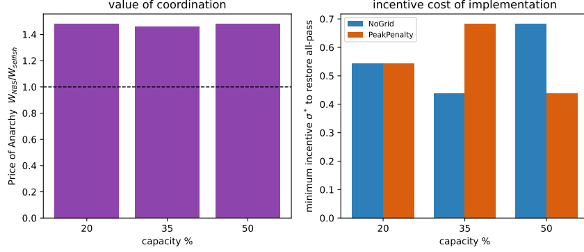
Figure 17: Left: price of anarchy W_{NBS}/W_{selfish} by capacity (coordination is worth roughly a 47% welfare gain). Right: minimum incentive \sigma^* that restores modelled all-pass, by capacity and grid policy.
