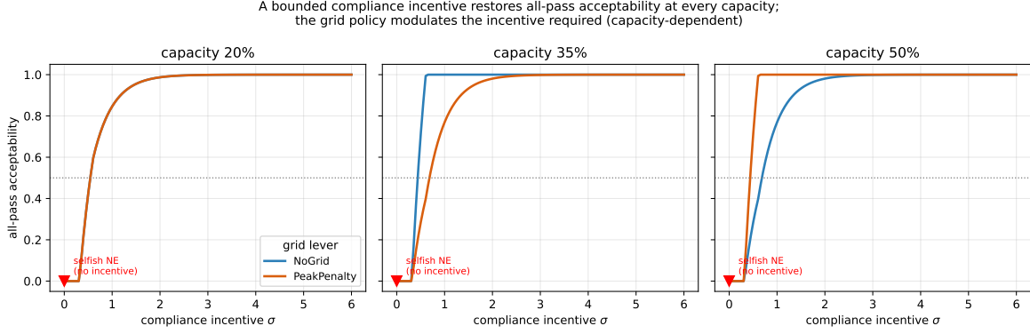
Figure 11: All-pass acceptability of the induced driver equilibrium as a function of the compliance incentive \sigma , for the two grid policies at each capacity. The selfish equilibrium ( \sigma = 0 , red marker) is unacceptable; a bounded incentive restores all-pass at every capacity. The grid policy modulates the incentive required, with a capacity-dependent sign (GridPeakPenalty helps at 50% capacity).
