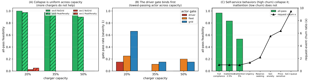
Figure 7: Disaggregated diagnosis. (A) All-pass feasibility by charger capacity and grid policy at full compliance (green) and severity 1 (red): the collapse is uniform across capacity, so infrastructure is not the lever. (B) Actor-gate pass rates by capacity at severity 1: the driver-service gate binds first (lowest-passing) across capacities, while the grid gate is healthiest at low capacity. (C) All-pass (bars) and request-event churn ratio (line) by behavior type: self-service behaviors (high churn, 1.3\text{--}9.5\times ) collapse feasibility and bind the driver gate, whereas mild inattention (low churn) does not.
