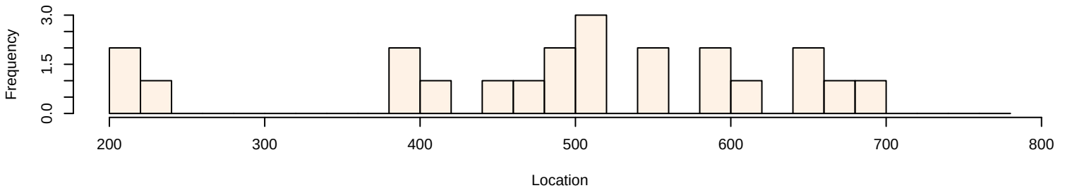
Histogram of detected change point 3
