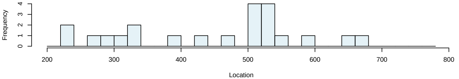
Histogram of detected change point 1
