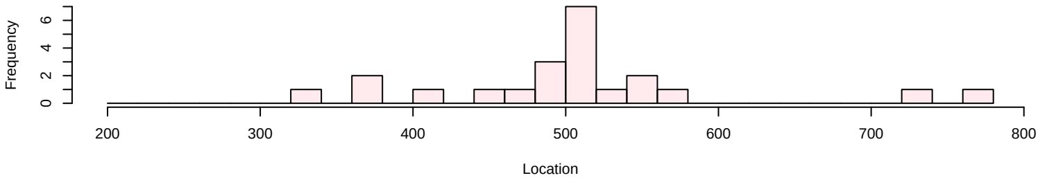
Histogram of detected change point 2
