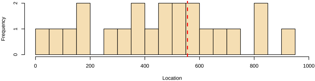
Histogram of detected change point 3
