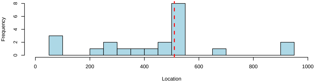
Histogram of detected change point 2
