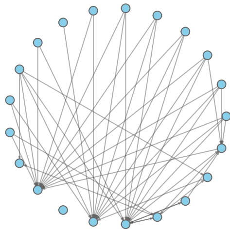
CP1 R cluster2
