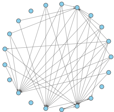
CP1 R cluster1
