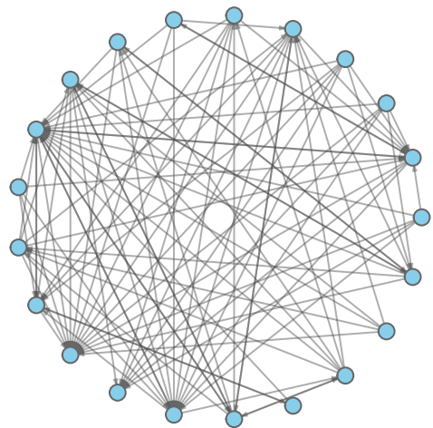
CP1 L cluster1
