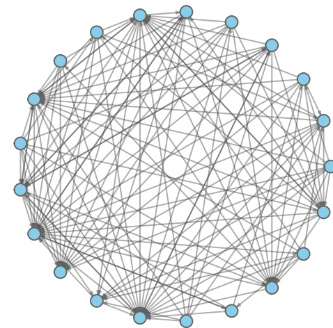
CP1 L cluster4
