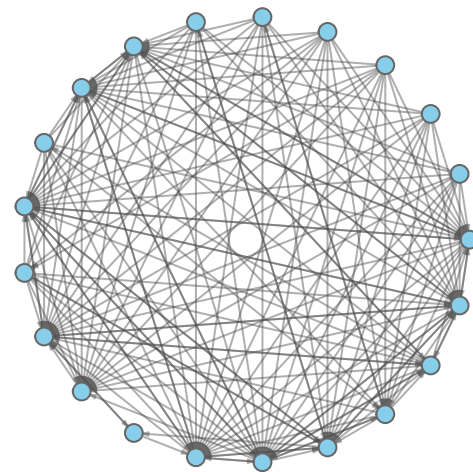
CP1 R cluster3
