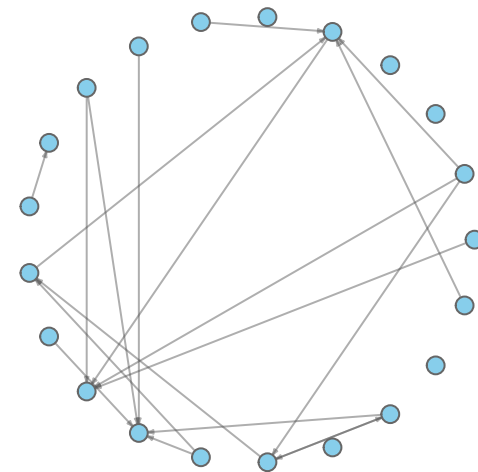
CP1 R cluster4
