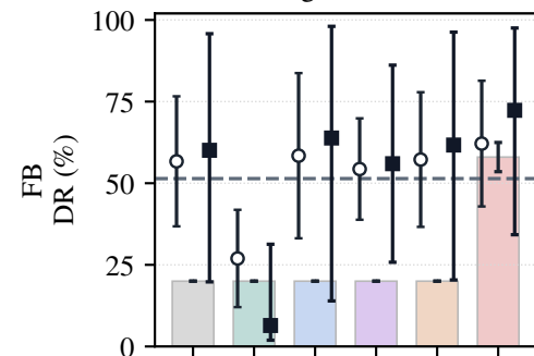
MagicGamma
