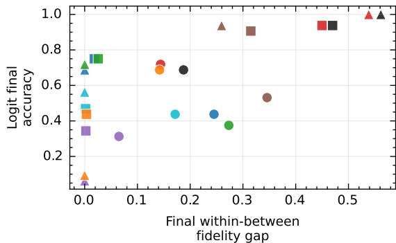
Synthetic eigengap
