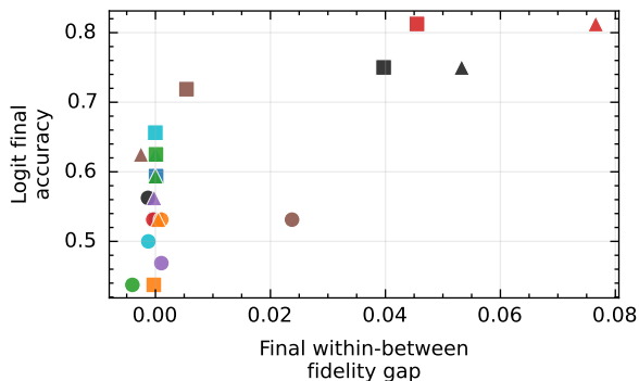
Synthetic eigengap
