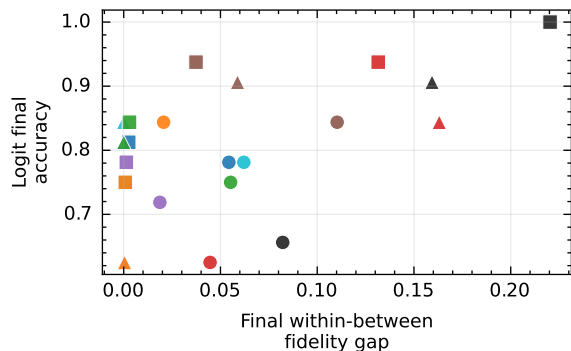
Synthetic singular
