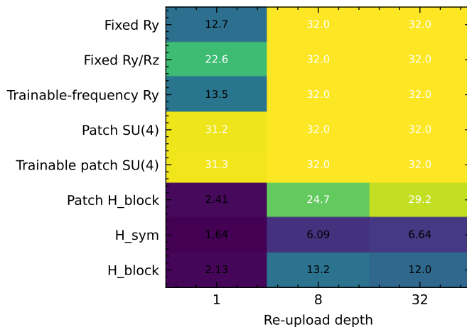
Synthetic eigengap
