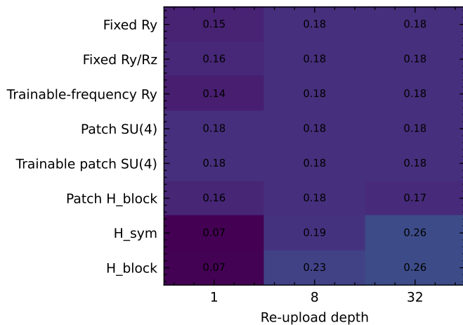
Synthetic eigengap
