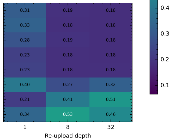
Synthetic singular
