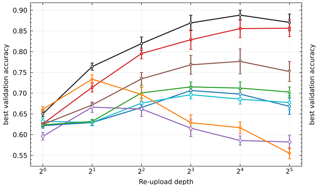
SYNTHETIC EIGENGAP
