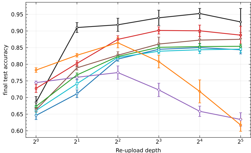
SYNTHETIC SINGULAR
