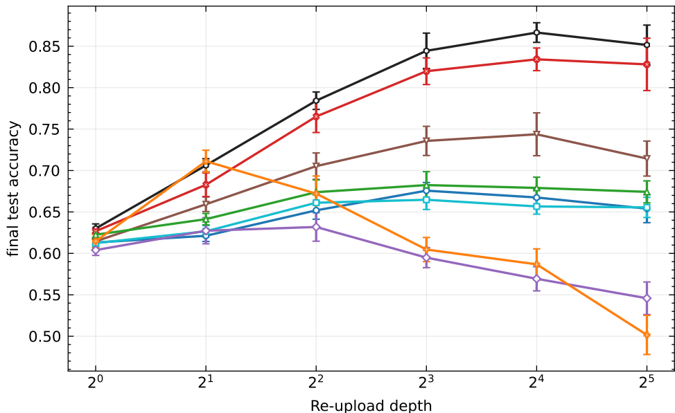
SYNTHETIC EIGENGAP
