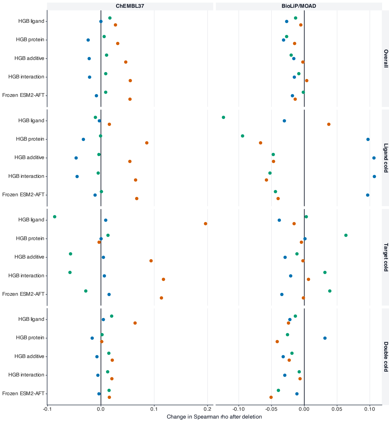
Largest-cluster deletion changes rank estimates
