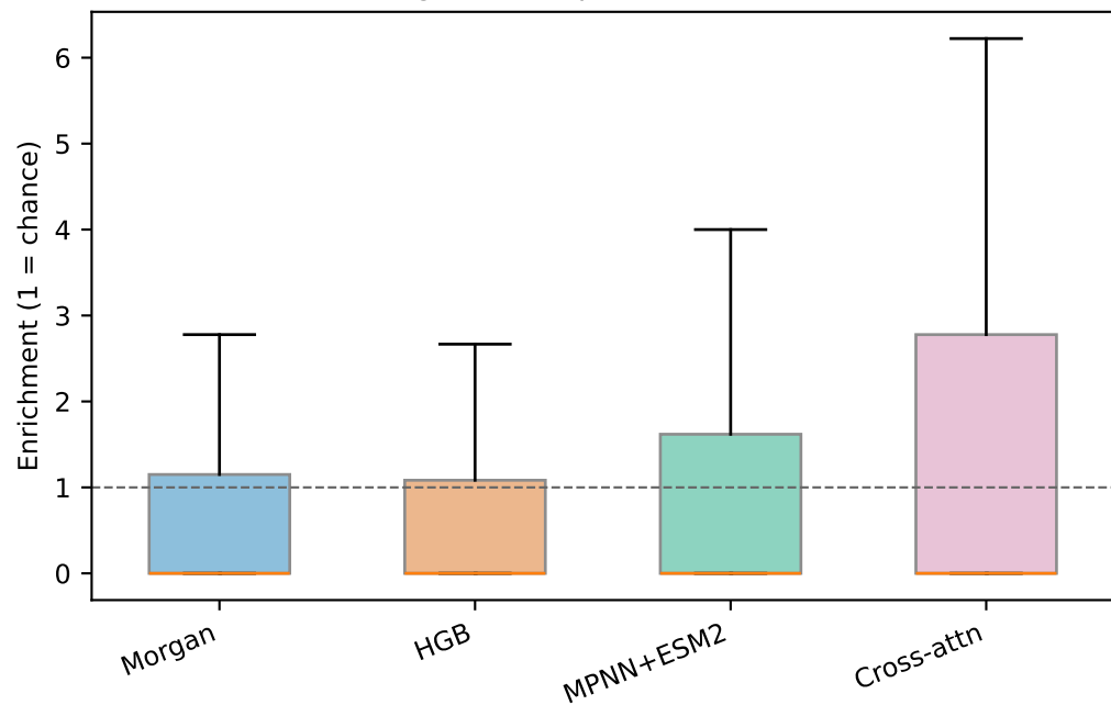
C Target-wise top-decile enrichment
