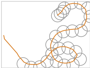
V3 LSTM
