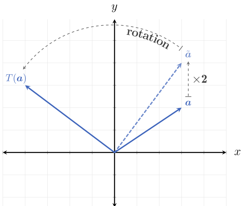
Figure 2.1: The transformation T applied to \mathbf{a} : first the vector is scaled by 2 in the y -direction, and then rotated by 90^\circ anti-clockwise.
