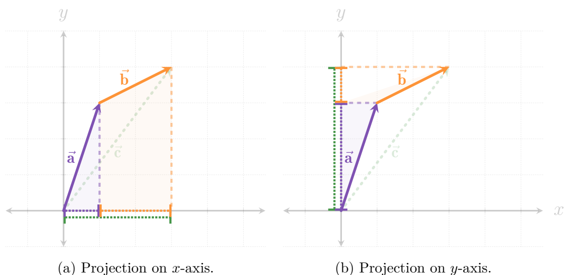
Figure 1.2: Projecting three vectors on the x - and y -axes: \vec{a} , \vec{b} and \vec{c} = \vec{a} + \vec{b} . Note how the projection of \vec{c} on to an axis is exactly the same as the addition of the projections of \vec{a} and \vec{b} on the same axis.
