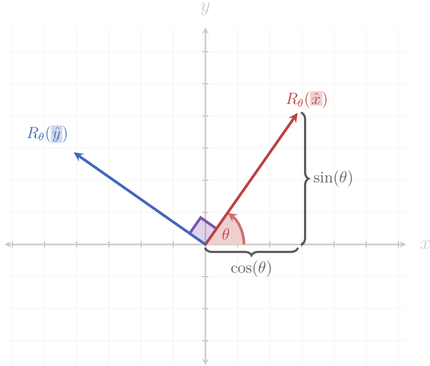
Figure 2.6: The two basis vectors \hat{x} , \hat{y} rotated by an angle \theta anti-clockwise around the origin. The coordinates of the rotated \hat{x} are simply the polar coordinates of a general vector which is at an angle \theta to the x -axis, with R = 1 (since \hat{x} is a unit vector).
