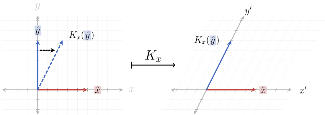
Figure 2.7: Shearing in the x -direction: while \hat{x} is kept untouched, \hat{y} is shifted by some value k \in \mathbb{R} .
