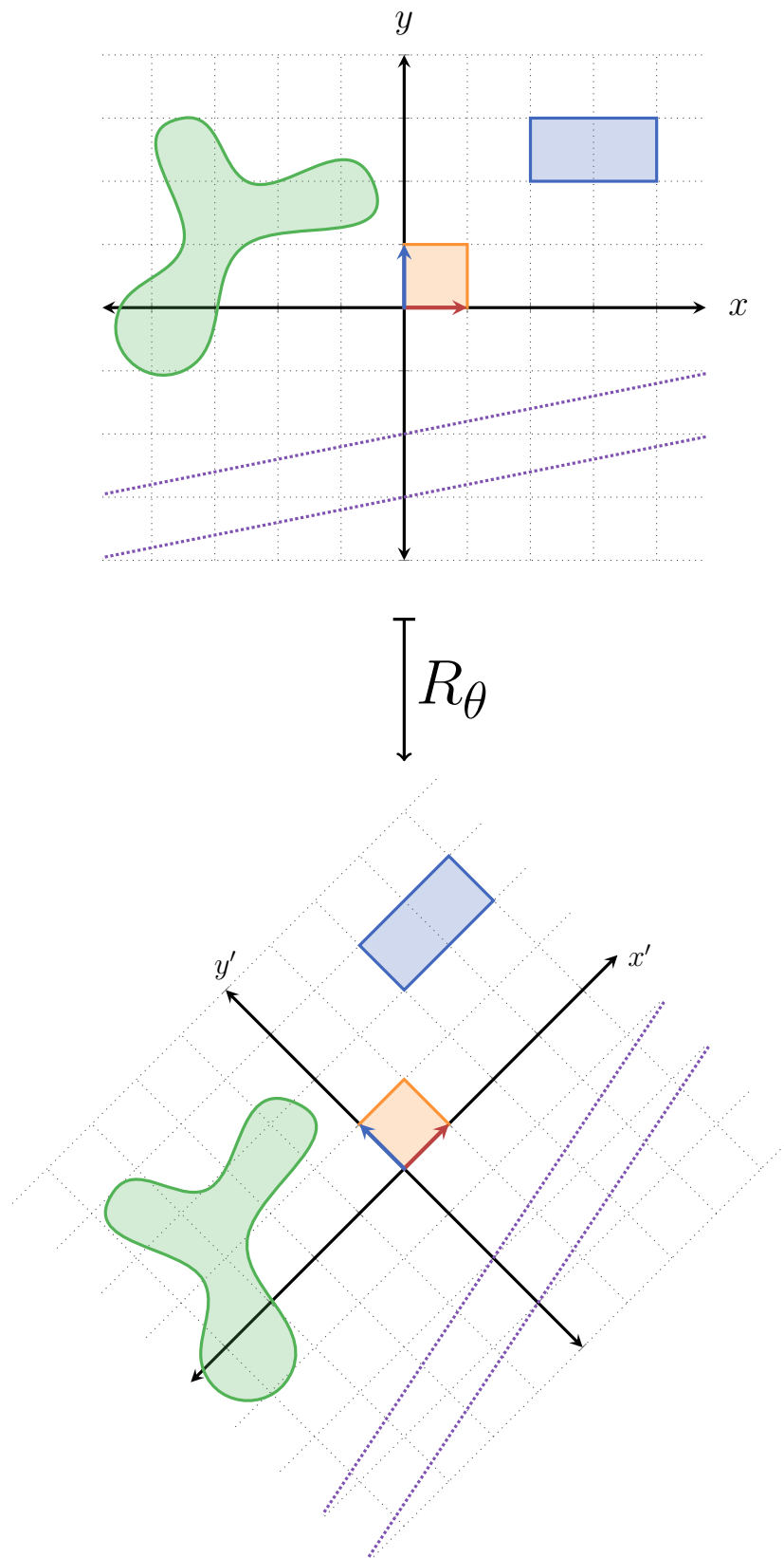
Figure 2.1: Testing a visualization idea for linear transformations.
