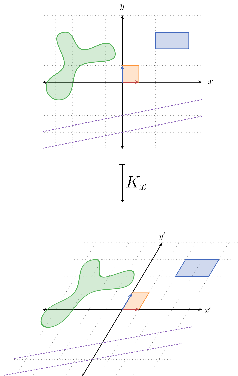
Figure 2.2: Testing a visualization idea for linear transformations... again.
