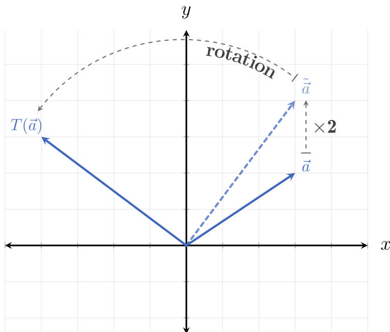
Figure 2.3: The transformation T applied to \vec{a} : first the vector is scaled by 2 in the y -direction, and then rotated by 90^\circ anti-clockwise.
