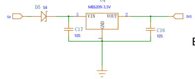
3.3V Power Supply Circuit
