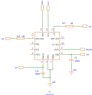
IMU Circuit
