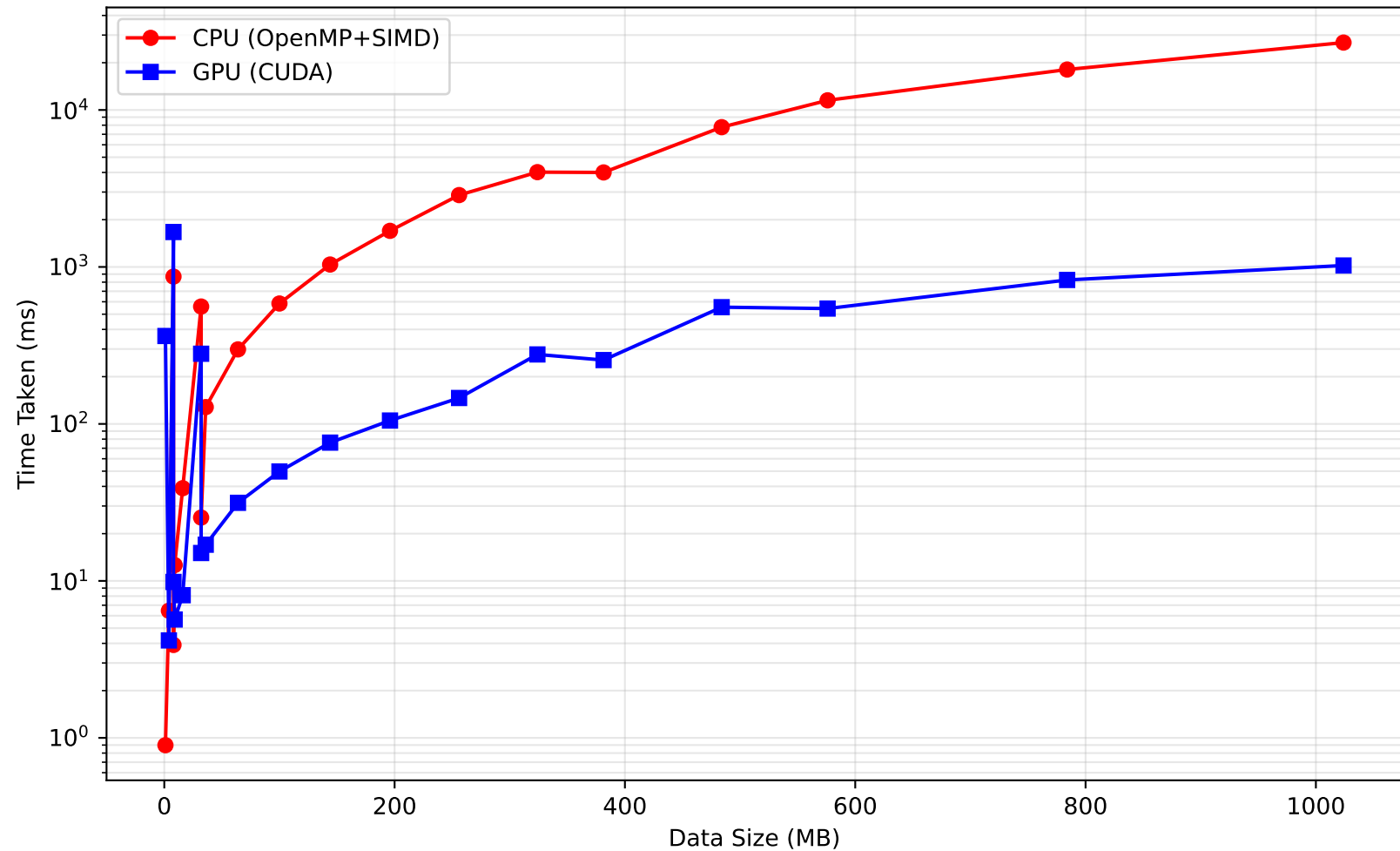
Scaling Performance: CPU vs GPU
