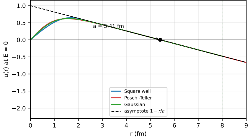
Figure 4: Three potentials tuned to the same (a, r_0) of the deuteron: the wavefunctions are identical outside the range and completely different inside . Dotted lines mark where each potential ends. Everything a low-energy experiment can see lives outside.
