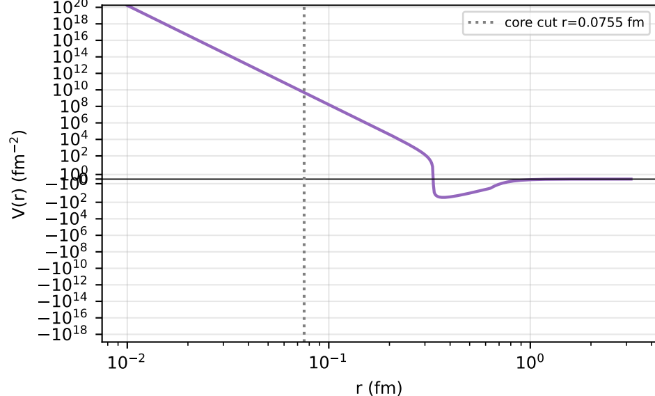
Fig. 1b — Lennard-Jones: hard core + vdW tail
