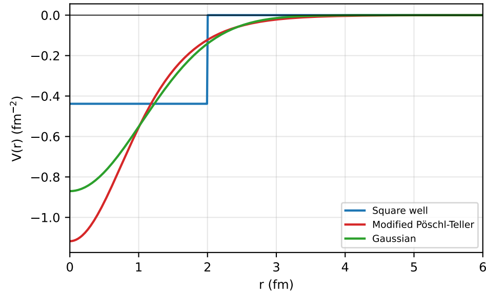
Fig. 2a — tuned to the deuteron a = 5.4 \text{ fm} , r_0 = 1.7 \text{ fm}
