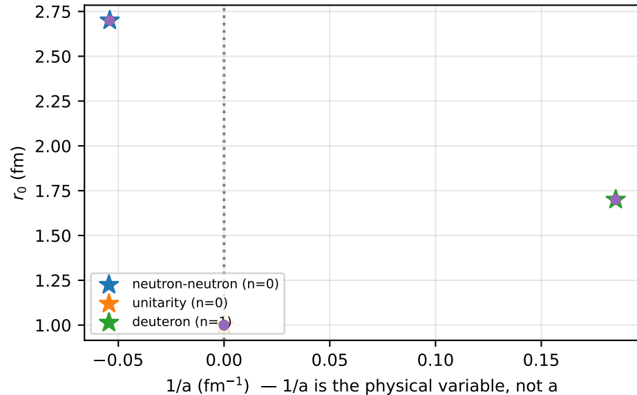
Fig. 2b — targets and solutions
