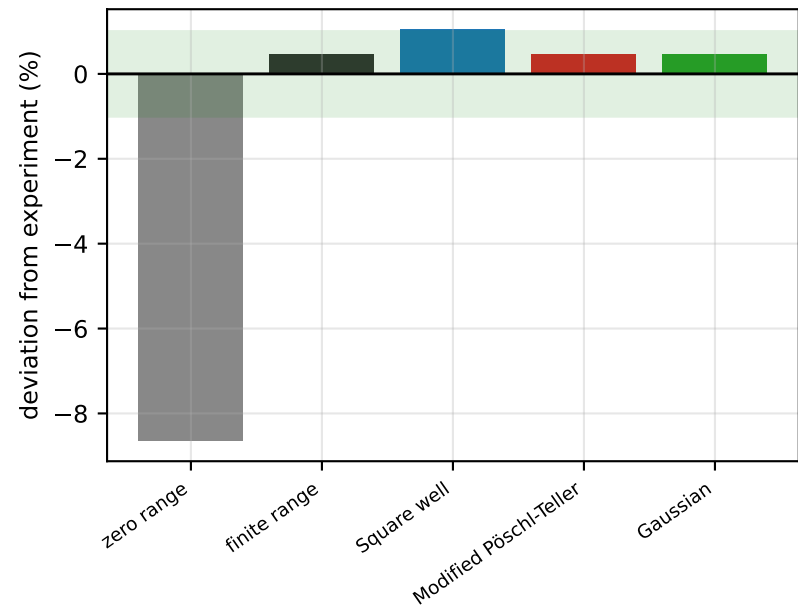
Fig. 3c — he4_dimer, |a|/r_0 = 11.3
