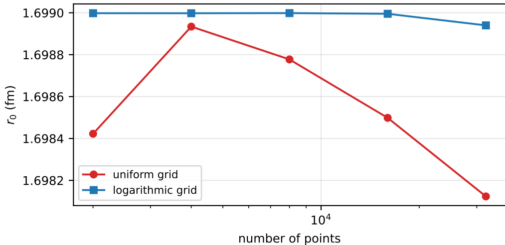
Lennard-Jones: convergence of r_0
