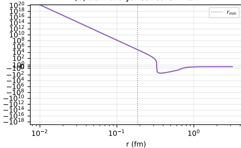
(b) Lennard-Jones: core + tail
