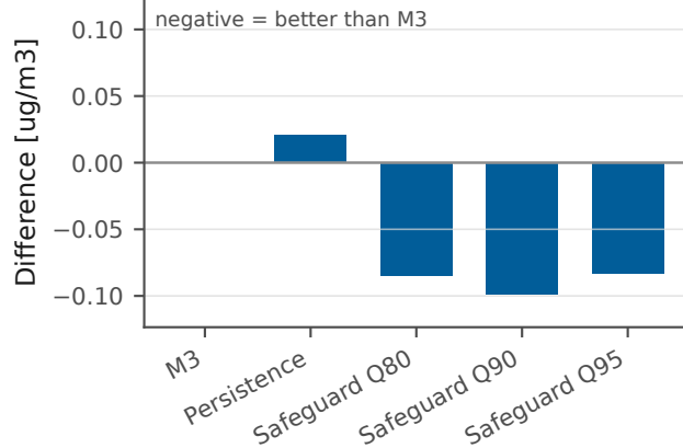
D. Full-test MAE difference vs M3
