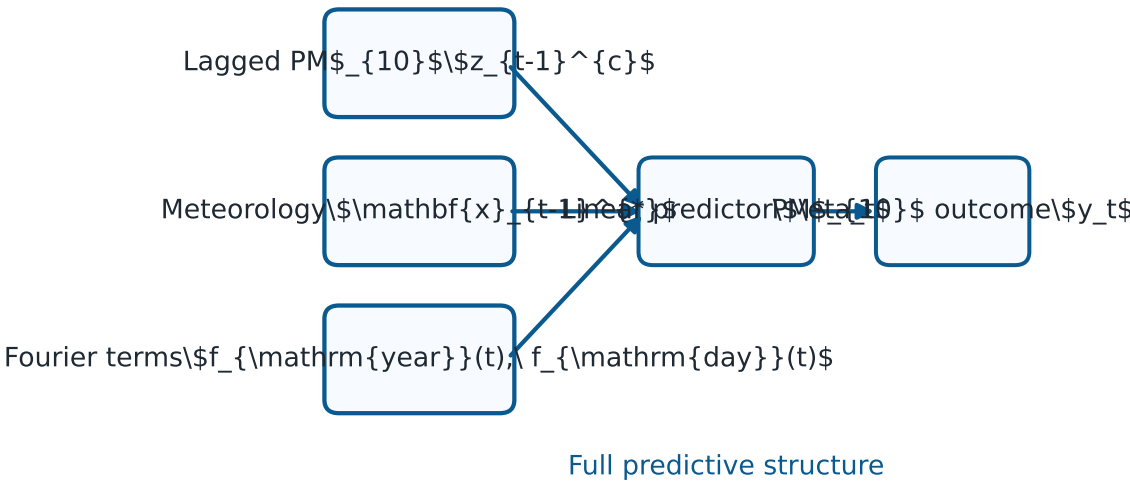
M3 Final model: lag + meteorology + seasonality
