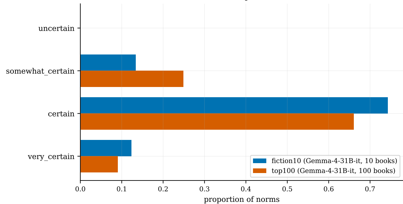
Confidence (qualitative) TVD=0.115 JSD=0.016
