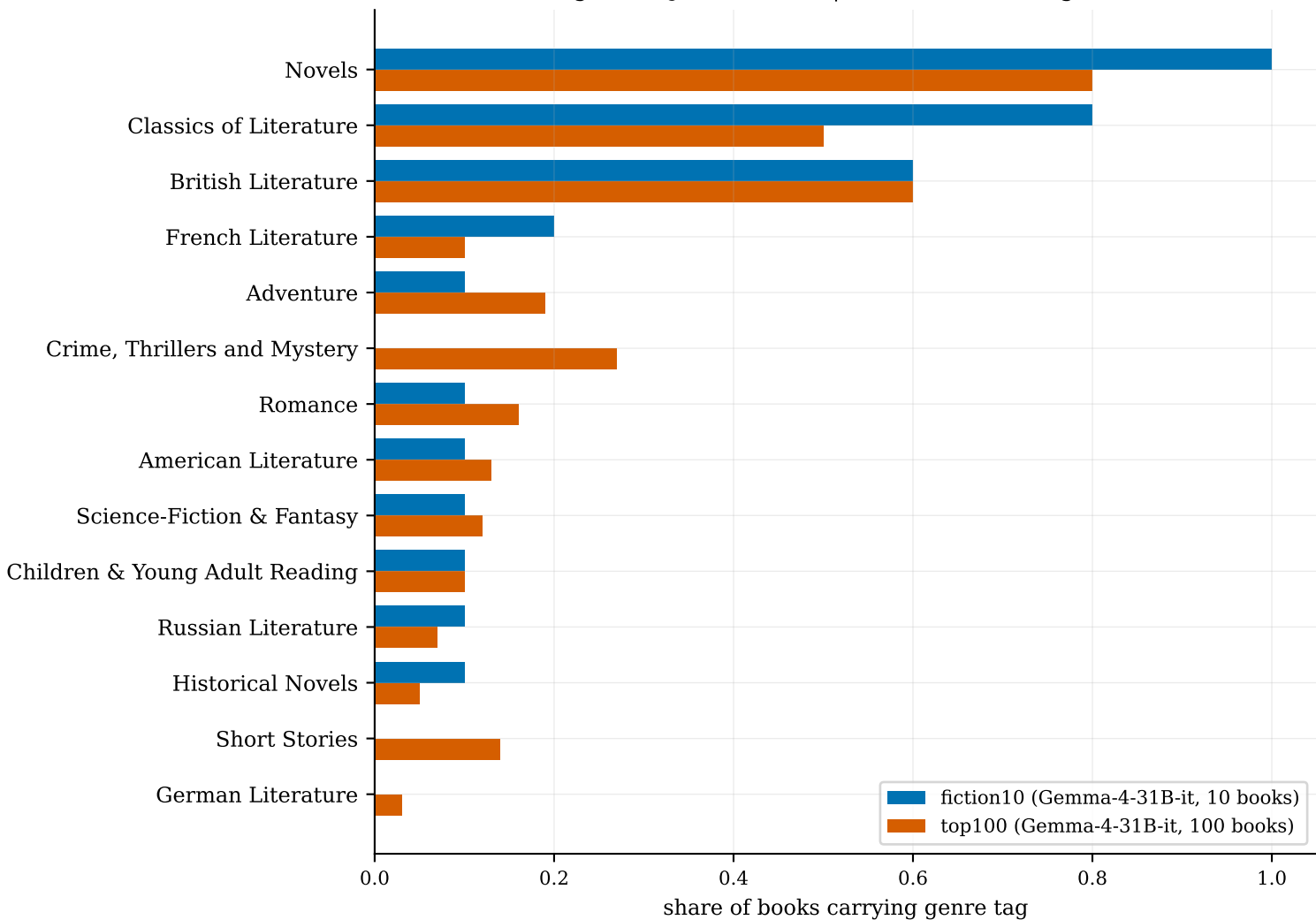
Genre (top 14 by pooled book share) tag-share JSD = 0.094 | 11 vs 17 distinct genres
