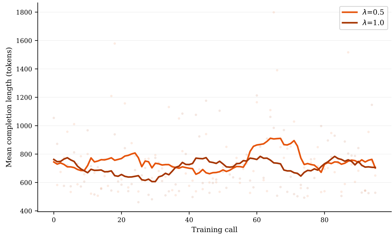
Completion Length Over Training (Qwen3.5-9B)
