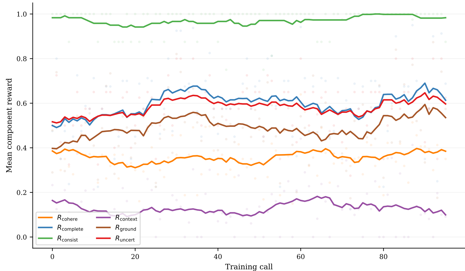
Per-Component Reward Decomposition ( \lambda = 0.5 )
