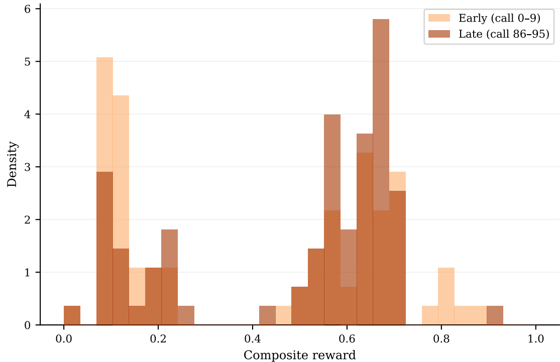
Reward Distribution Shift ( \lambda=0.5 )
