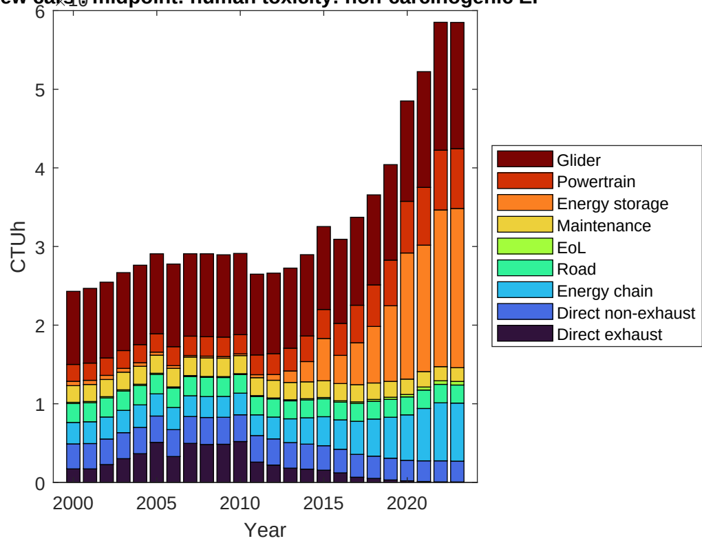
New cars midpoint: human toxicity: non-carcinogenic EF
