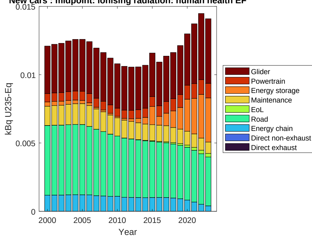
New cars : midpoint: ionising radiation: human health EF
