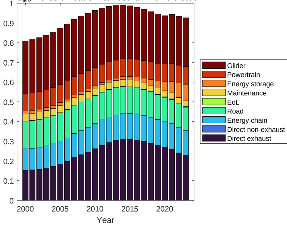
Midpoint: acidification: terrestrial : vehicle stock
