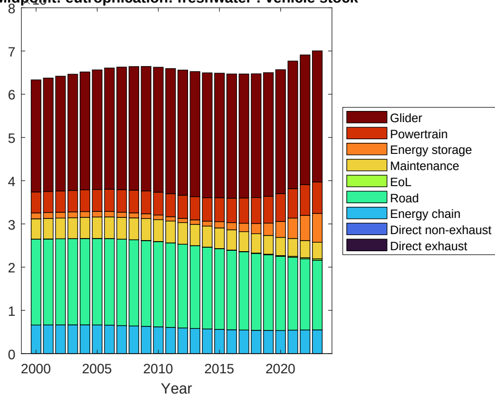
Midpoint: eutrophication: freshwater : vehicle stock
