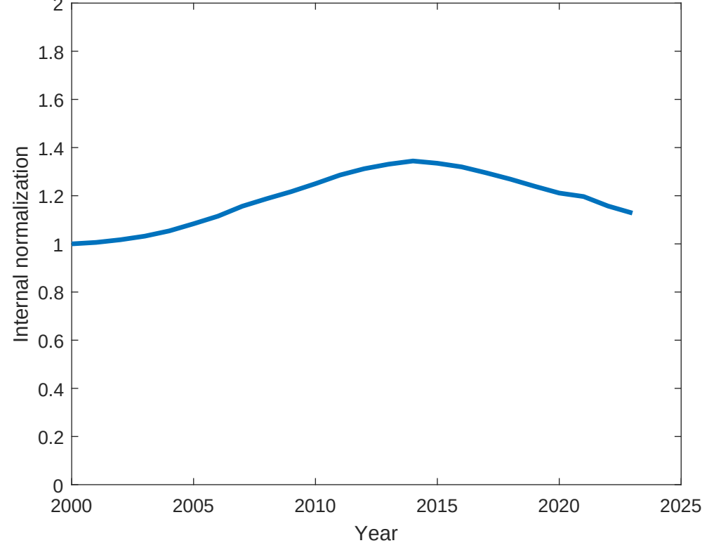
Midpoint: photochemical oxidant formation: human health EF : vehicle stock
