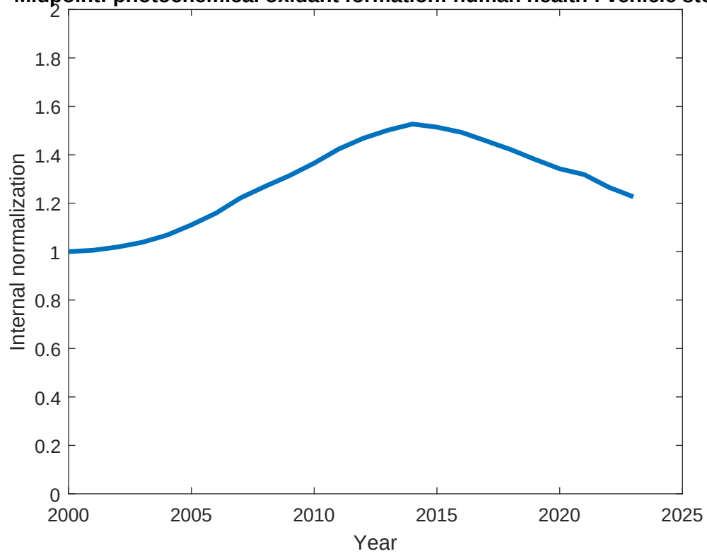
Midpoint: photochemical oxidant formation: human health : vehicle stock
