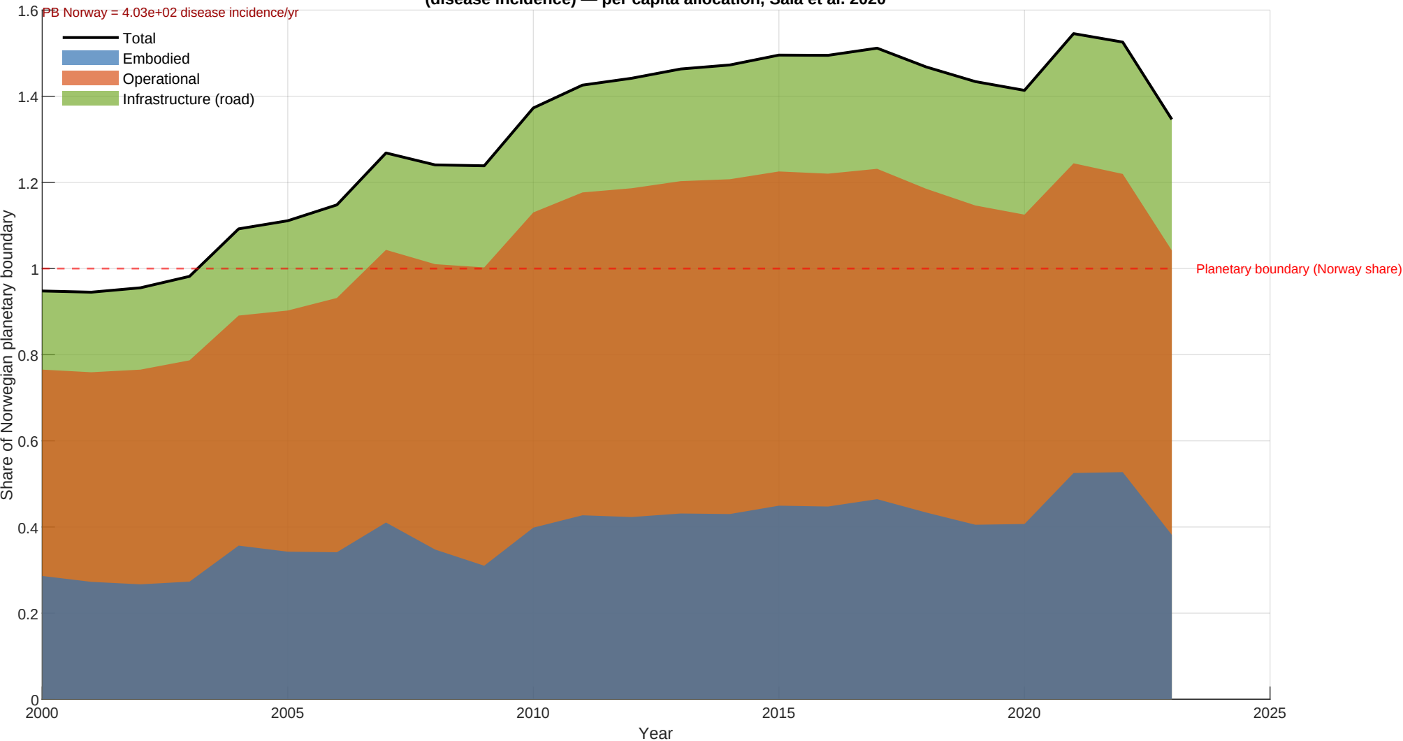
EF v3.1 : particulate matter formation (disease incidence) — per capita allocation, Sala et al. 2020
