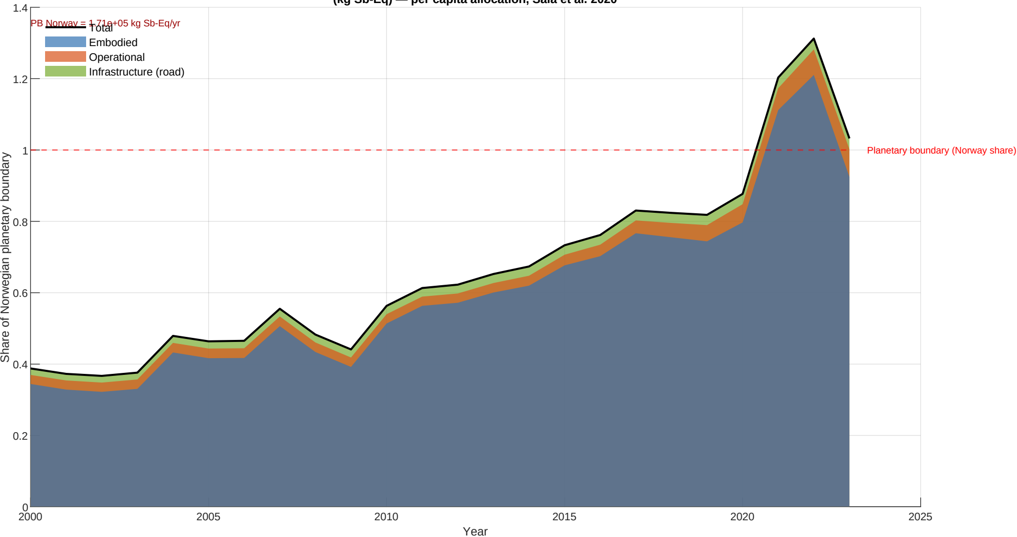
EF v3.1 : material resources: metals/minerals (kg Sb-Eq) — per capita allocation, Sala et al. 2020
