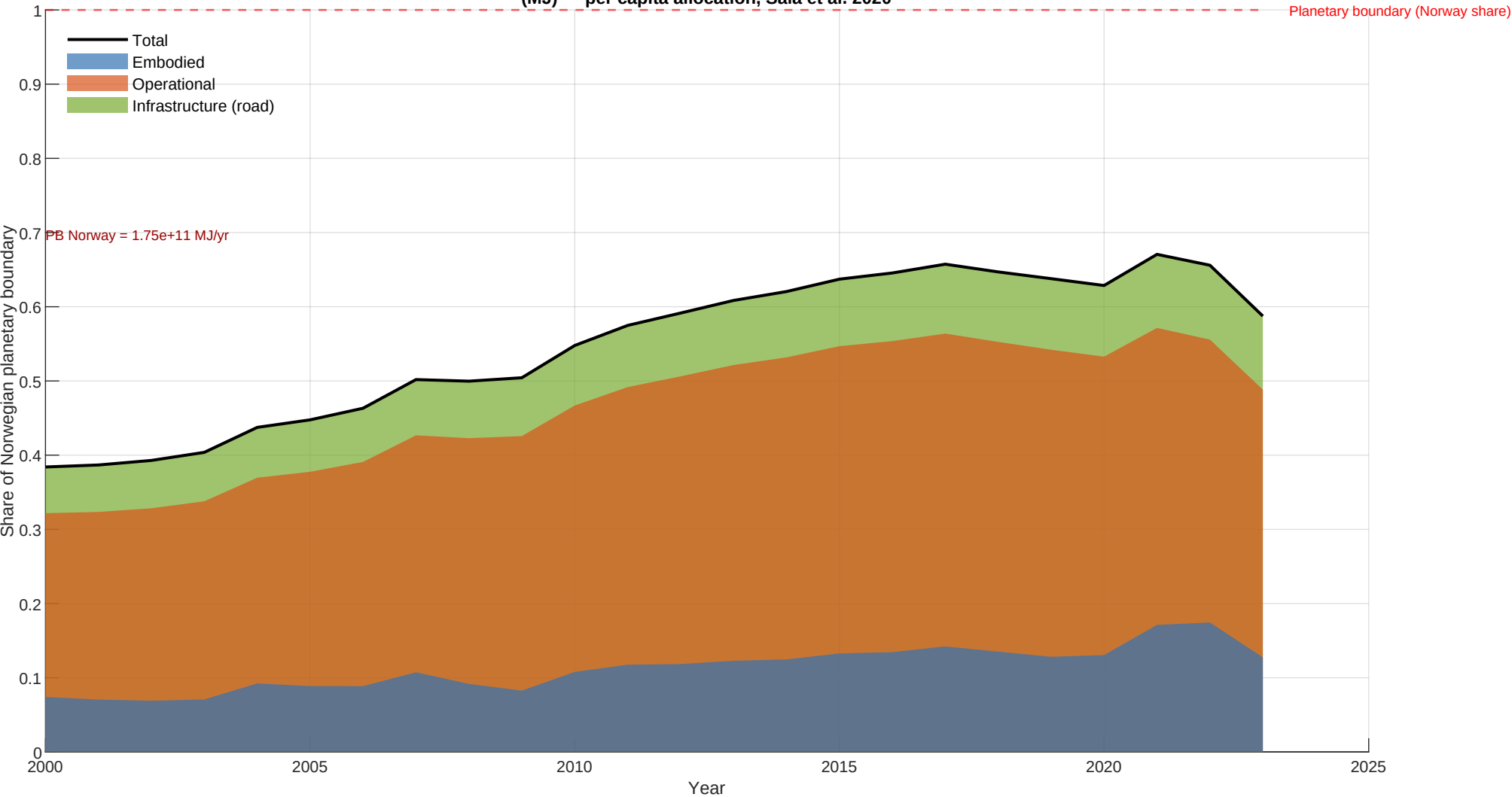
EF v3.1 : energy resources: non-renewable (MJ) — per capita allocation, Sala et al. 2020
