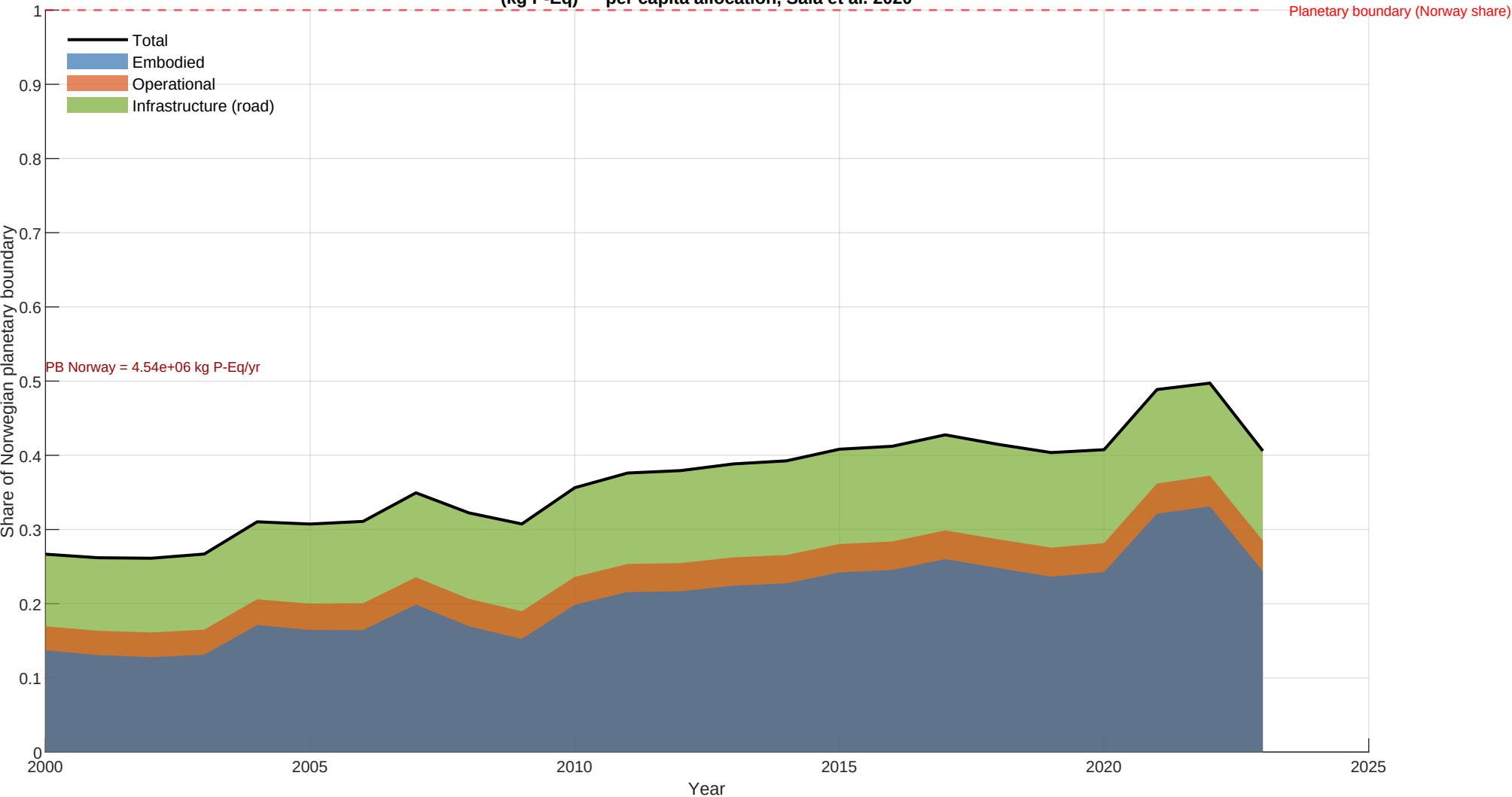
EF v3.1 : eutrophication: freshwater (kg P-Eq) — per capita allocation, Sala et al. 2020
