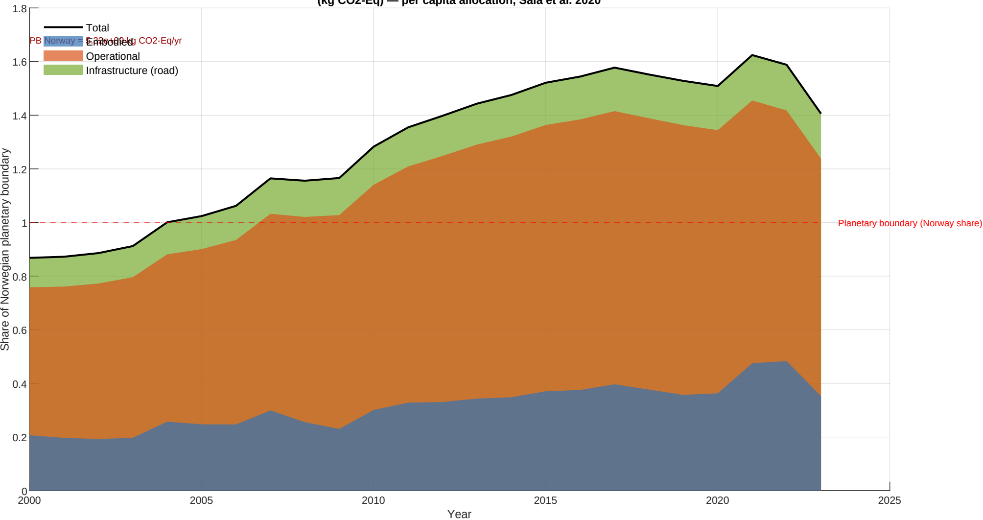
EF v3.1 : climate change (kg CO 2 -Eq) — per capita allocation, Sala et al. 2020
