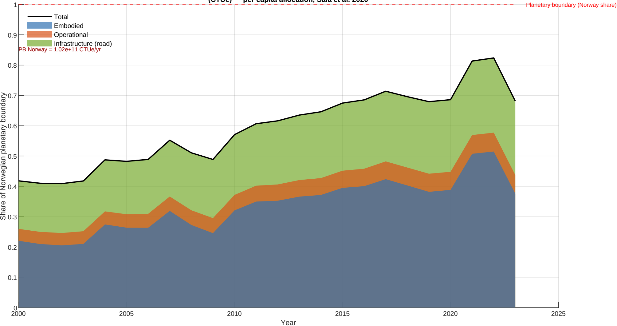
EF v3.1 : ecotoxicity: freshwater (CTUe) — per capita allocation, Sala et al. 2020
