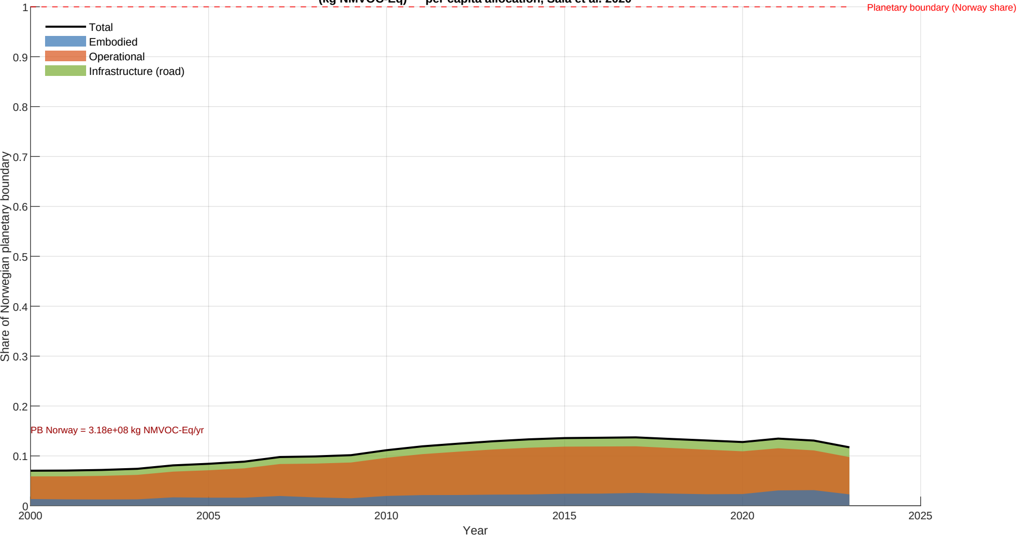
EF v3.1 : photochemical oxidant formation: human health (kg NMVOC-Eq) — per capita allocation, Sala et al. 2020
