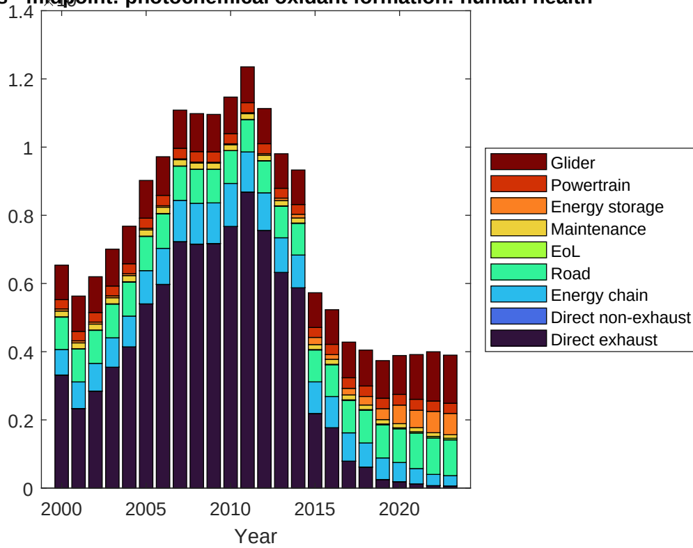
New cars - midpoint: photochemical oxidant formation: human health
