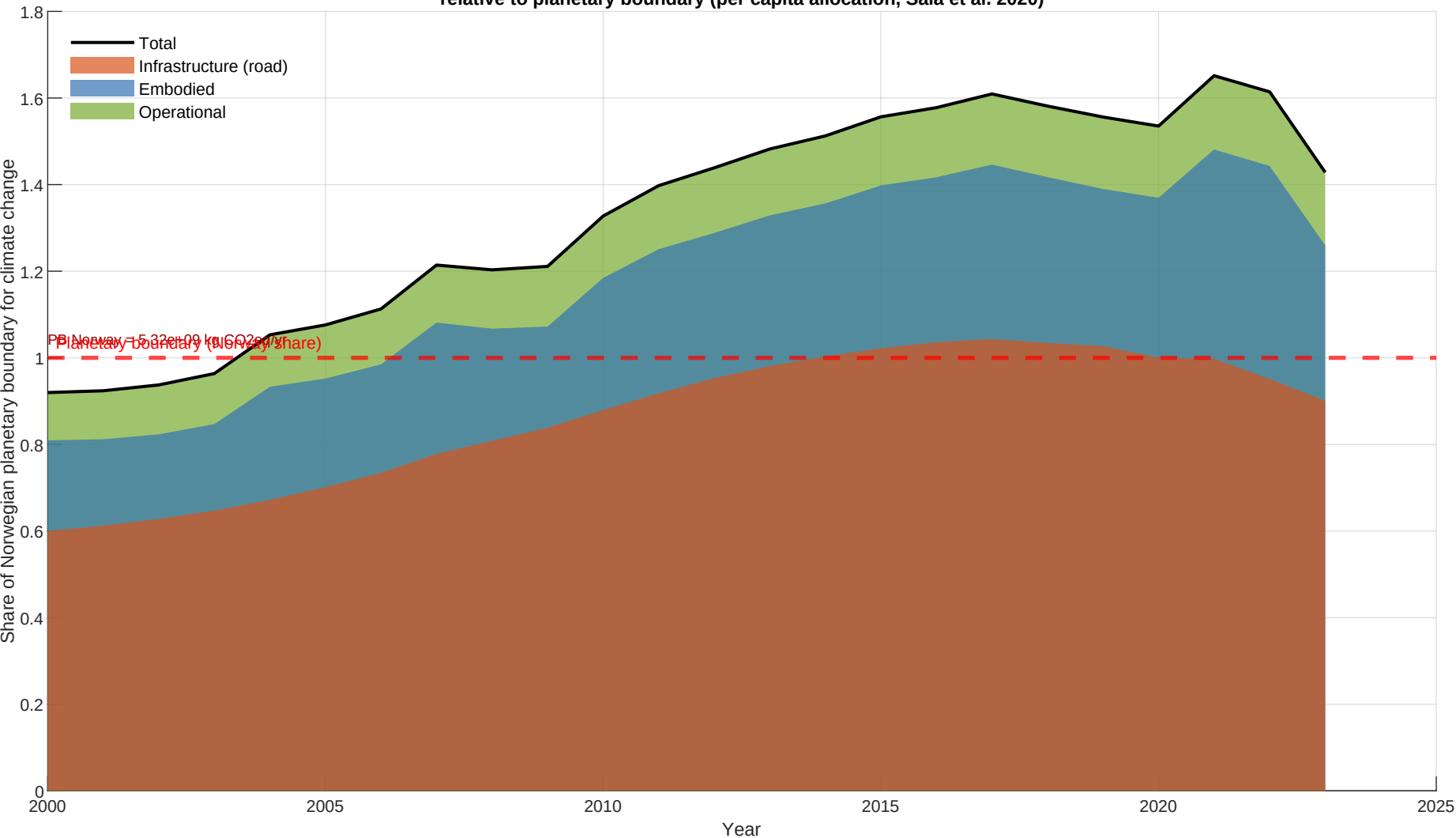
Norwegian fleet : Climate change impact relative to planetary boundary (per capita allocation, Sala et al. 2020)
