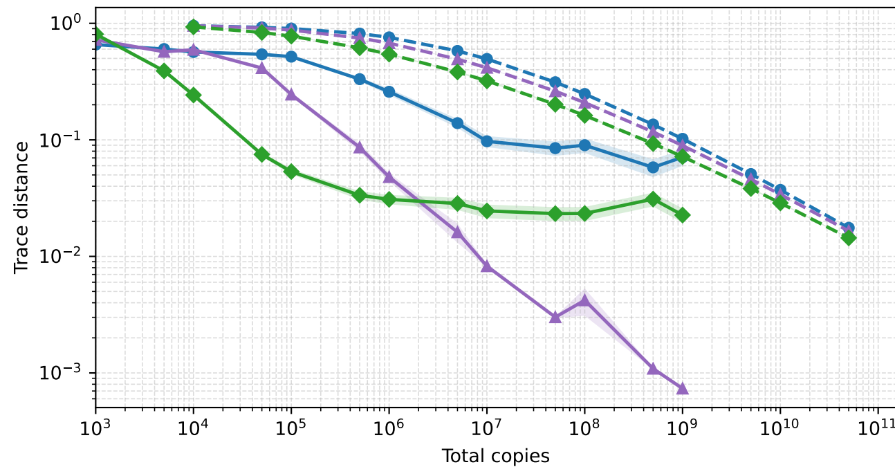
Reconstruction error vs. total copies ( n = 8 ; d = 1, 2, 3 )
