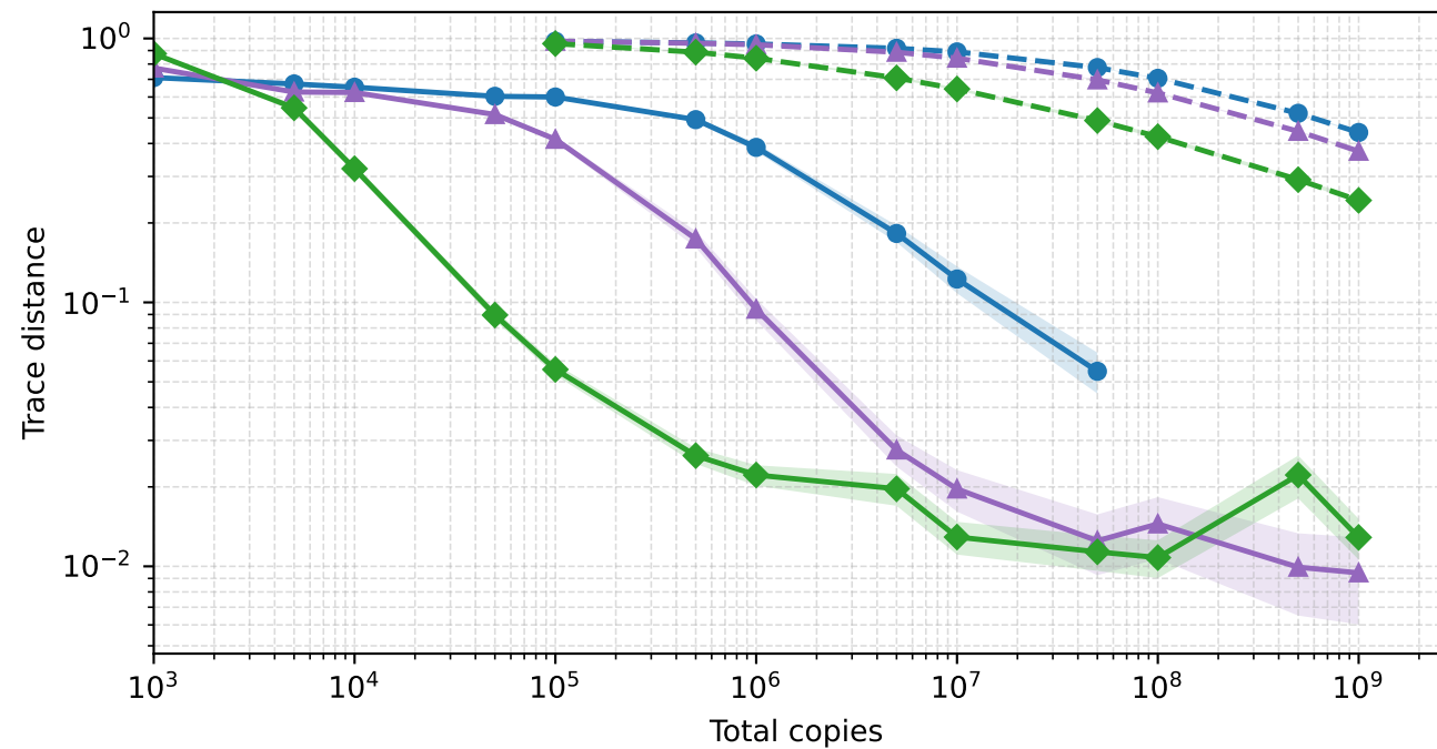
Reconstruction error vs. total copies ( n = 10 ; d = 1, 2, 3 )
