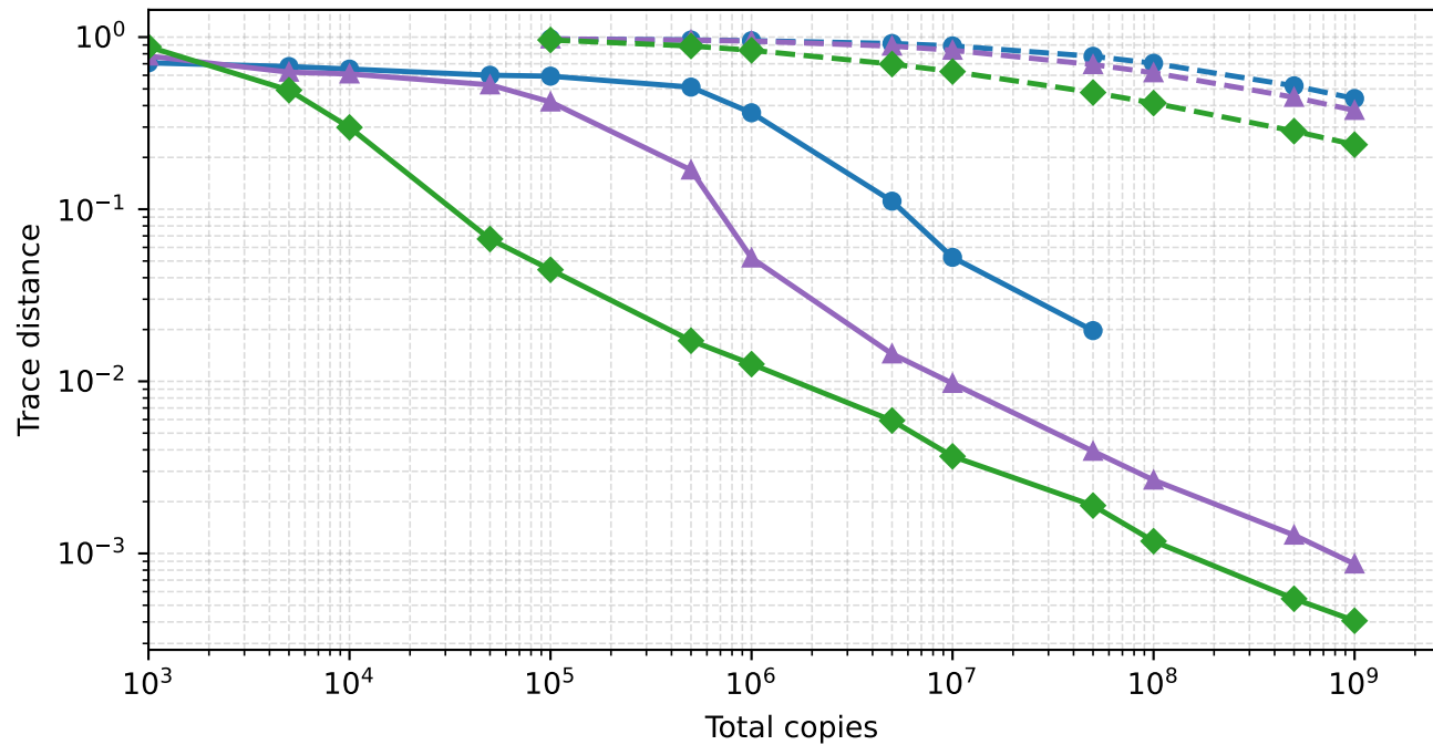
Median reconstruction error vs. total copies ( n = 10 ; d = 1, 2, 3 )
