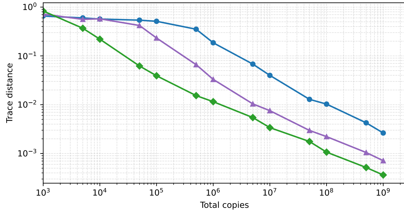
Median reconstruction error vs. total copies ( n = 8 ; d = 1, 2, 3 )
