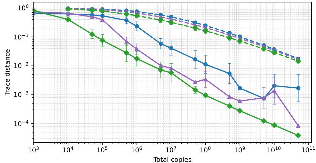
Reconstruction error vs. total copies ( n = 8 ; all-seed/state mean; log-SD bars)
