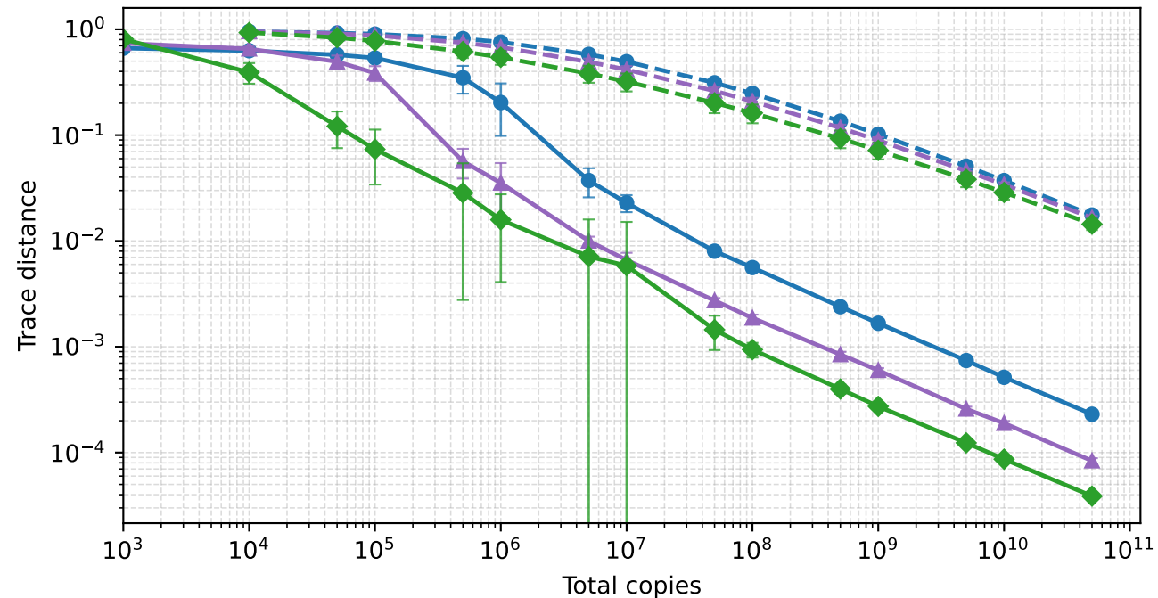
Reconstruction error vs. total copies ( n = 8 ; median-seed/state mean)
