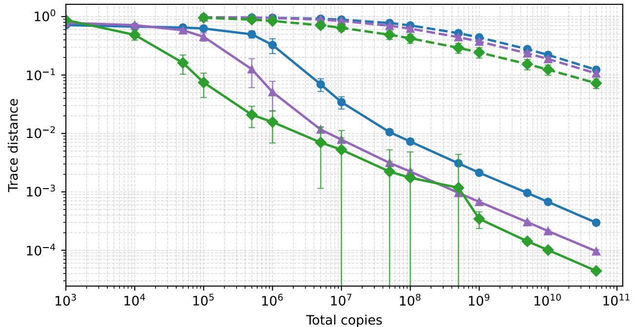
Reconstruction error vs. total copies ( n = 10 ; median-seed/state mean)
