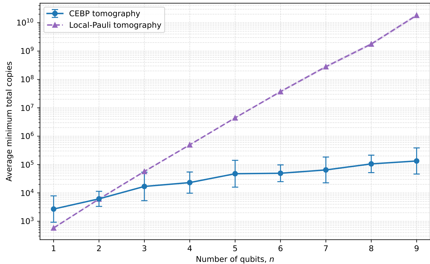
Average minimum total copies vs. number of qubits ( D_{\text{tr}} \leq 0.05 )
