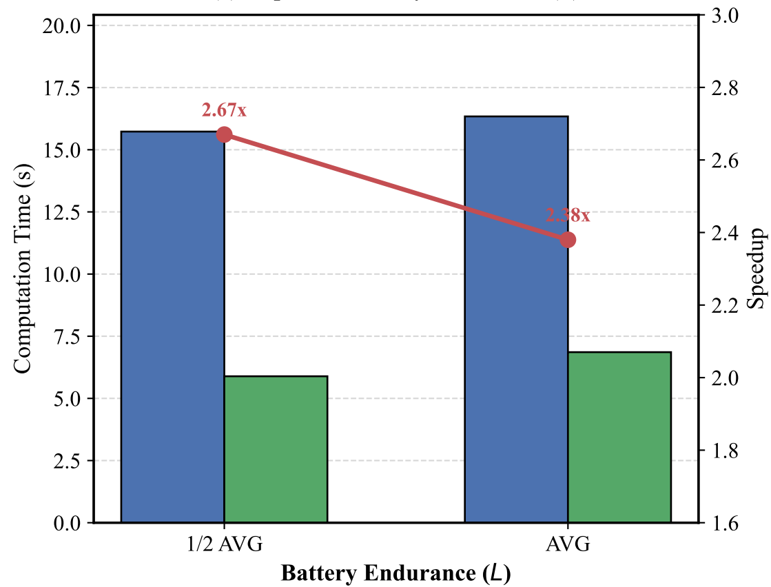
(c) Impact of Battery Endurance ( L )
