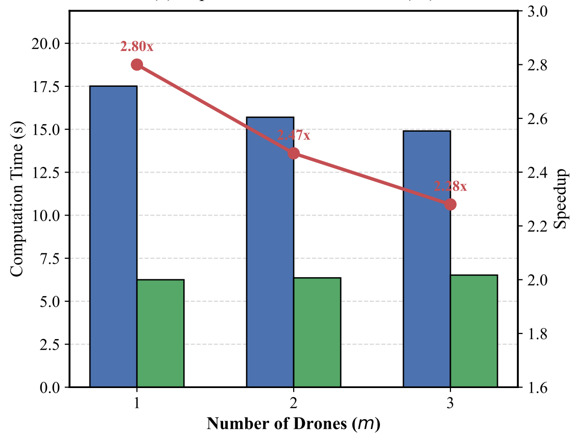
(b) Impact of Number of Drones ( m )
