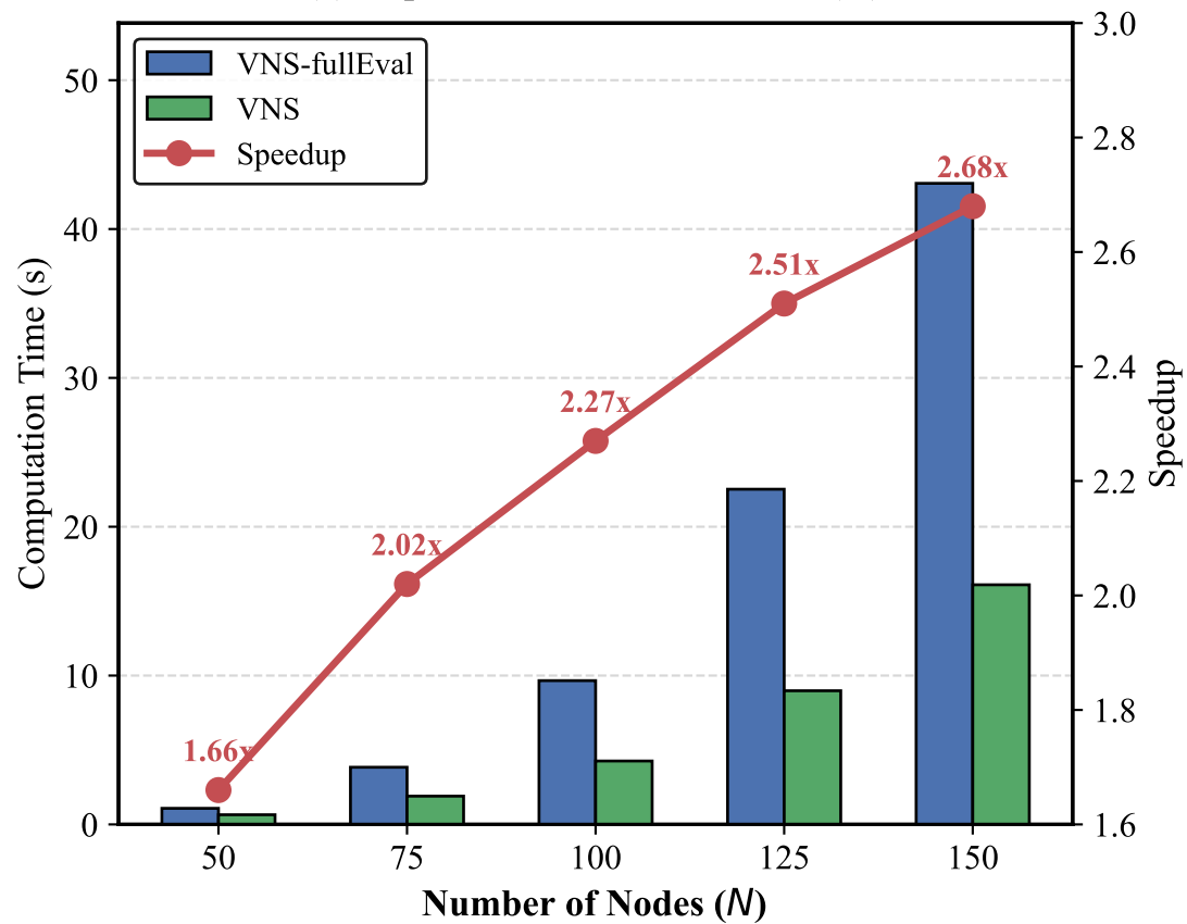
(a) Impact of Number of Nodes ( N )
