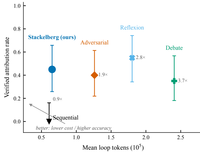
Figure 5: Verified attribution versus mean loop-token cost across the five Exp-B methods ( n=20 shared frozen blackboards each; error bars: Wilson 95% CIs). Stackelberg sits on the efficient frontier at the lowest token cost; adversarial matches its point estimate only at 1.9\times the cost, and the external multi-call protocols cost 2.8\times (Reflexion) to 3.7\times (Debate). Reflexion’s higher point estimate (0.55 vs 0.45) is not significant — its interval overlaps Stackelberg’s over most of its range (0:2 discordant pairs, p = 0.5 ).
