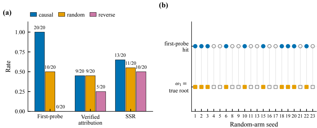
Figure 3: Exp-A commitment-order ablation and alignment audit (measured; snapshot mode; n=20/\text{order} ; plant me_force_zero_sea ). (a) First-probe hit, verified attribution, and SSR@ K by probe order. (b) Seed-level alignment audit of the random arm: a first-probe hit occurs if and only if the committed shuffle places the guilty layer first ( \omega_1 = a^* ; 10/10 with zero exceptions) — the random arm’s naming performance is carried entirely by accidental alignment with the ranking. Seeds 7, 12, 14 had no completed run manifest and are outside the campaign’s n=20 .
